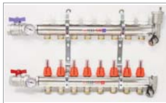
NP Brass Manifold
